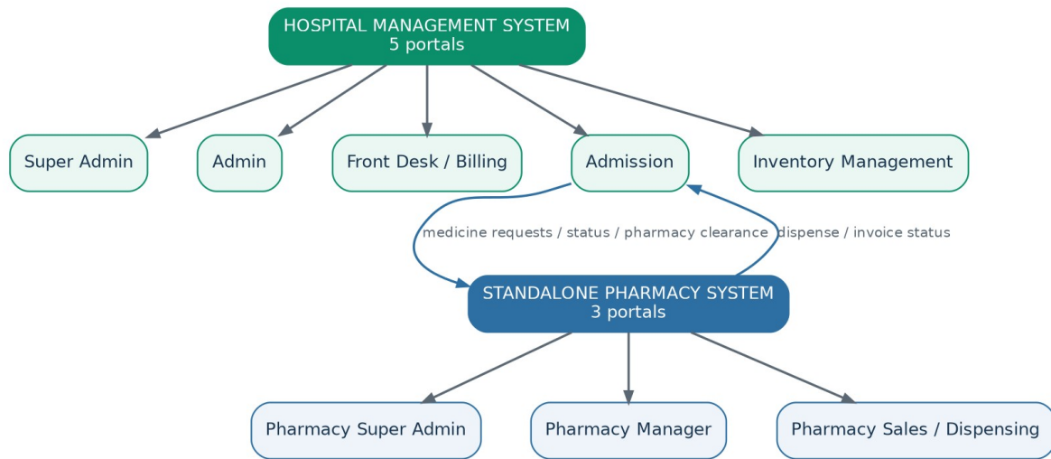
Overall HMS + standalone Pharmacy boundary.
