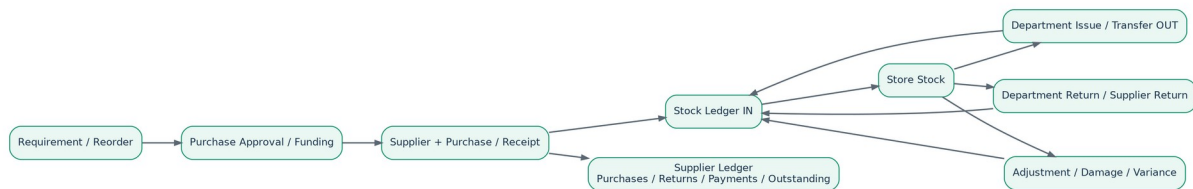
HMS Inventory purchase, stock ledger, supplier ledger and issue flow.
